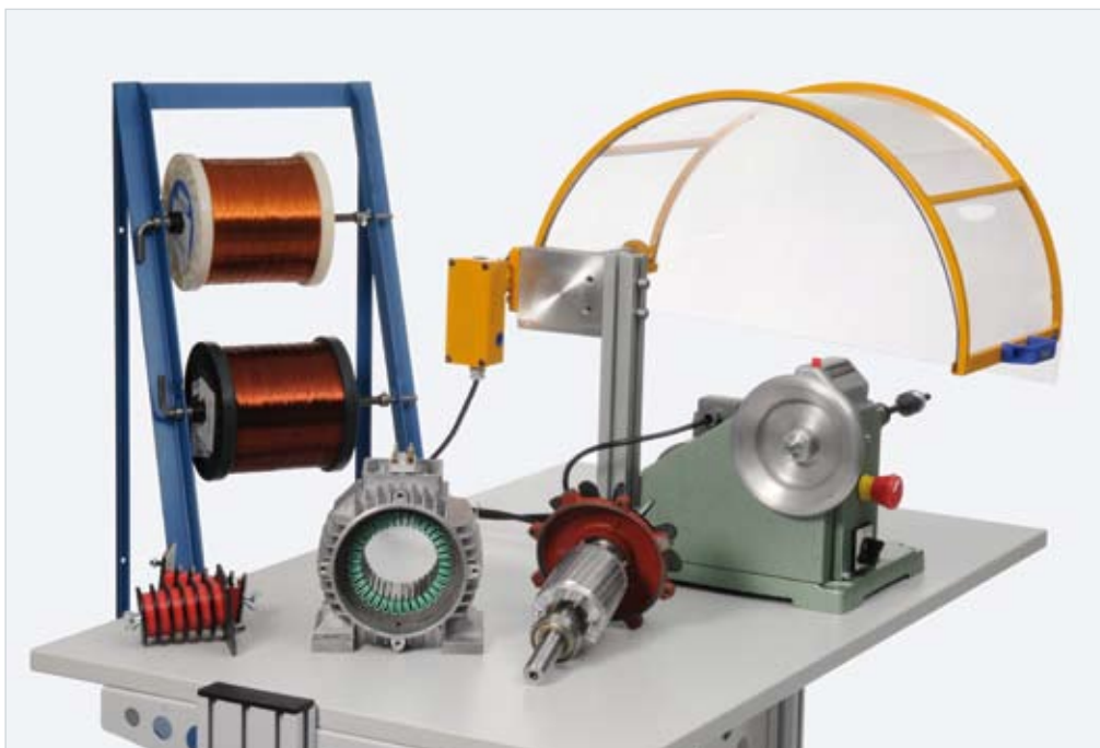
Experiment example: "Winding electrical machine coils EMW 20"
