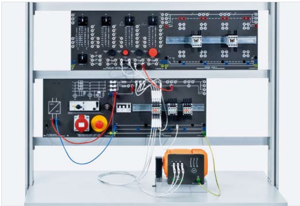
Experiment example: "Contactor circuits in three-phase EST 2"
