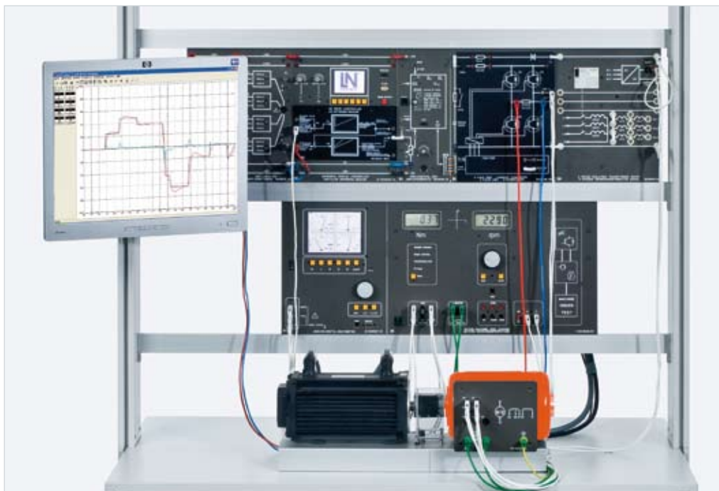
Experiment example: "Converter drives with DC motor EPE 21"
