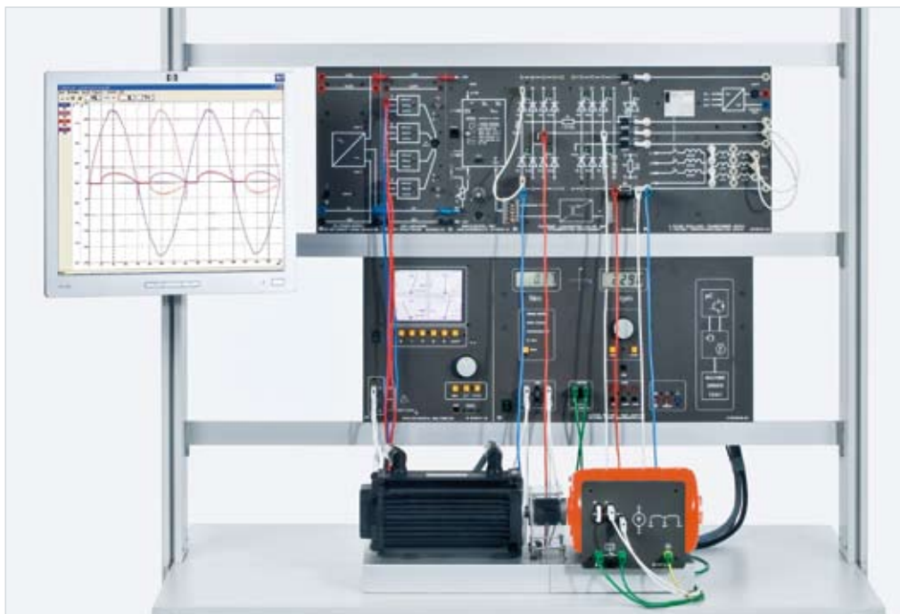
Experiment example: "Converter drives with universal motor EPE 16"
