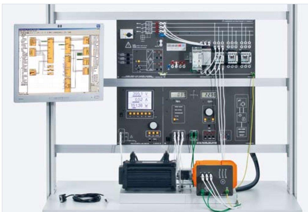
Experiment example: "Motor management relays EDT 51"
