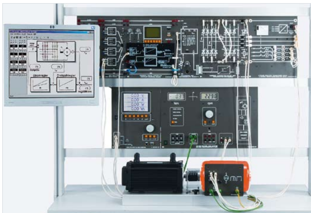
Experiment example: "Converter drives with DC motors EPE 11"
